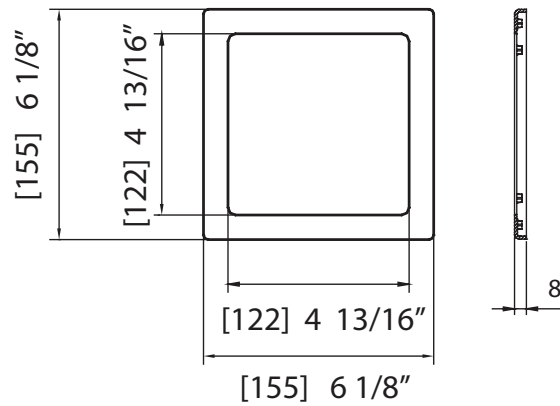
Speaker cover
